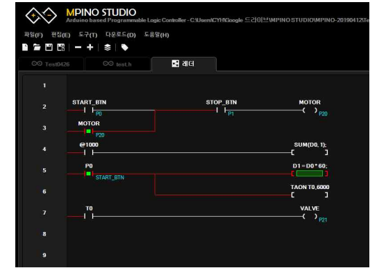
[ LADDER LOGIC ]
